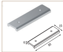
48V-Q2 ALUMINIUM CONNECTION
