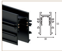
48V-Q2 RECESSED TRIMLESS HIGH RAIL
