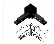
48V-Q2 CONNECTOR HIGH
