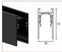
48V-Q2 SURFACE HIGH TRACK RAIL
