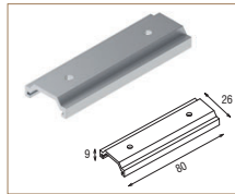
48V-Q1 ALUMINIUM CONNECTION
