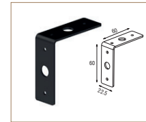
48V-Q2 ANGLE CONNECTION BRACKET
